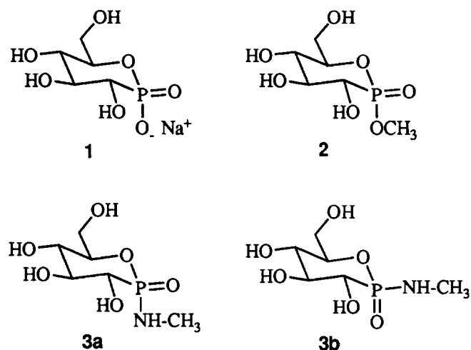
Figure 1. Structures of cyclic phosphonate and phosphonamidate analogues of glucose.
