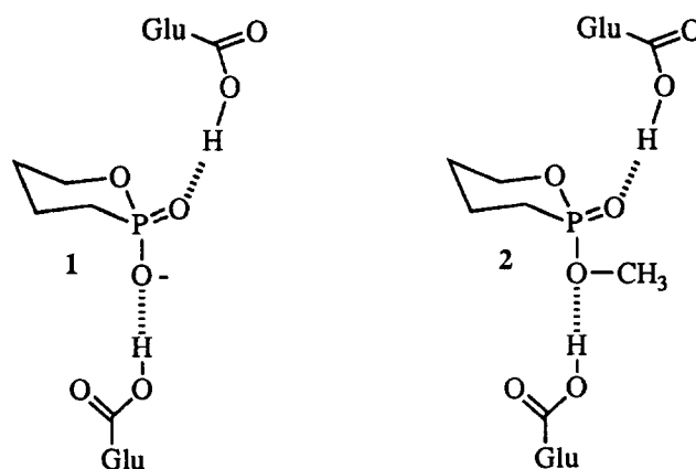
Figure 4. Proposed binding of phosphonate analogues to an inverting glycosidase. Dashed lines indicate hydrogen bonding interactions.
