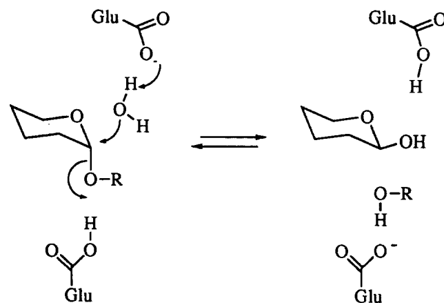
Figure 2. General mechanism for an inverting glycosidase.
