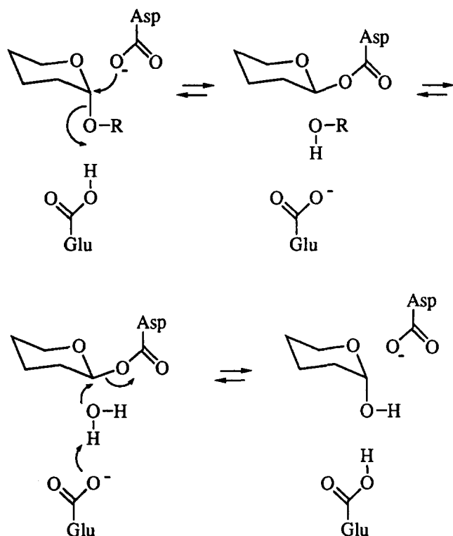
Figure 3. General mechanism for a retaining glycosidase.
