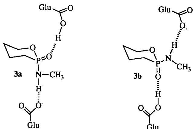
Figure 5. Proposed binding of stereoisomeric phosphonamidate analogues to an inverting glycosidase. Dashed lines indicate hydrogen bonding interactions.
